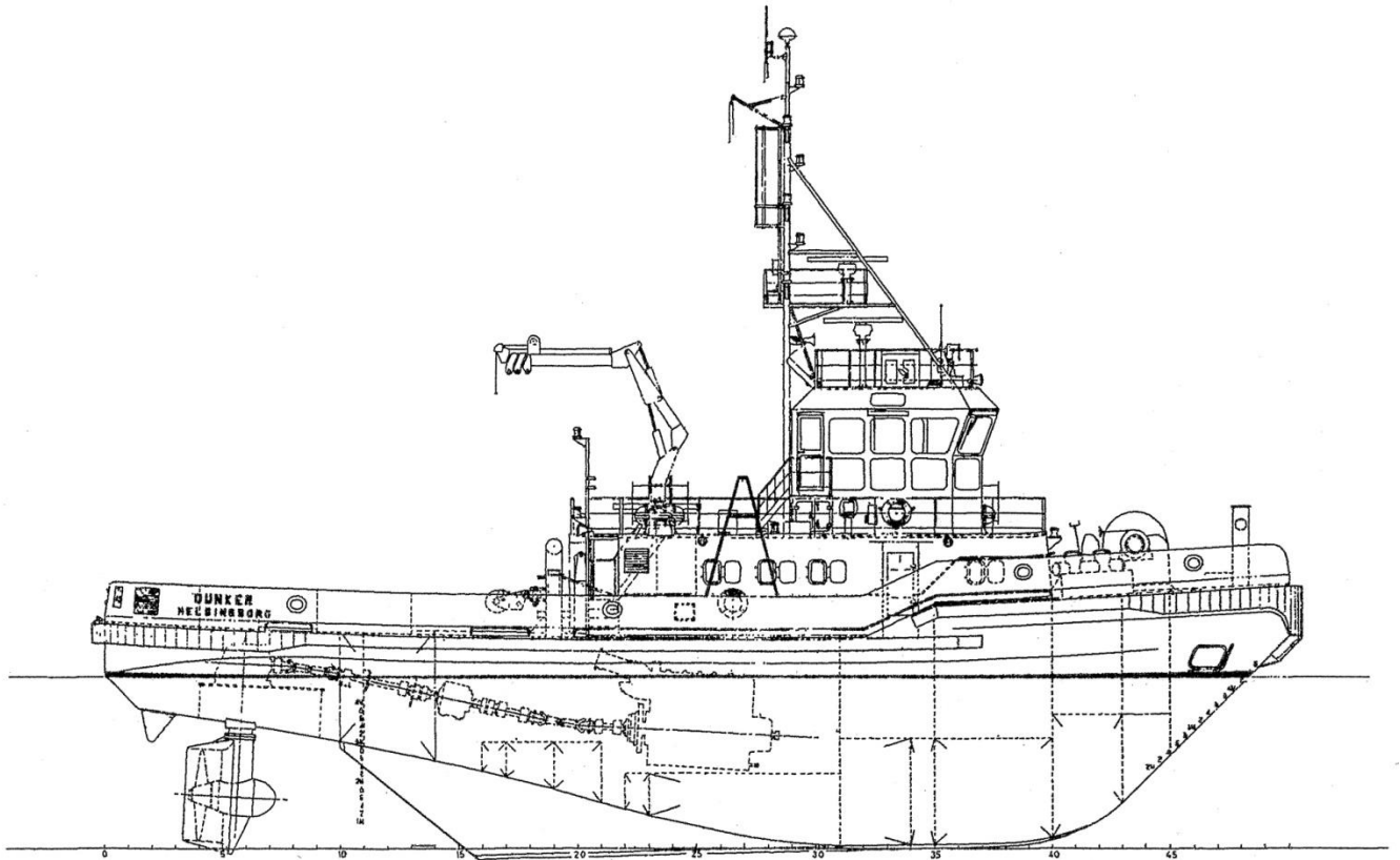
SIDE VIEW
